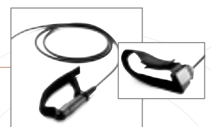
The SAVOX® R-C300 offers two alternative remote Push-To-Talk solutions, the "riot-ptt" and the "rifle-ptt".
